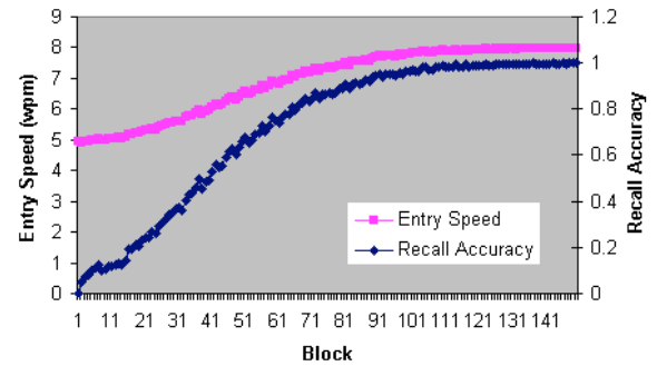
Figure 4: Simulated Entry Speed (in wpm - words per minute) and the recall accuracy (0 to 1) over 150 blocks as the simulated user transitions from novice to expert level. The simulated user reaches the expert level at around 111 th block.
