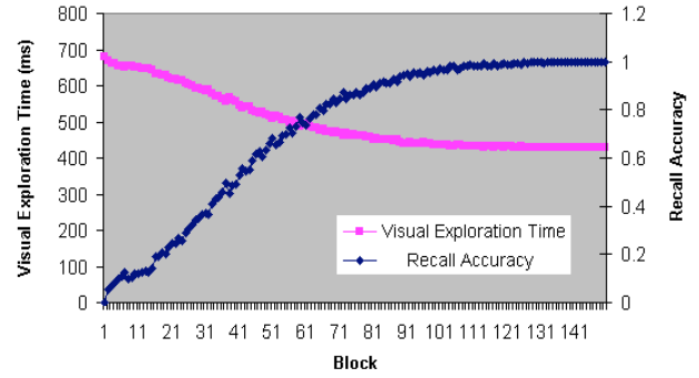
Figure 3: Simulated visual exploration time (in ms) and the recall accuracy (0 to 1) over 150 blocks as the simulated user transitions from novice to expert level.
