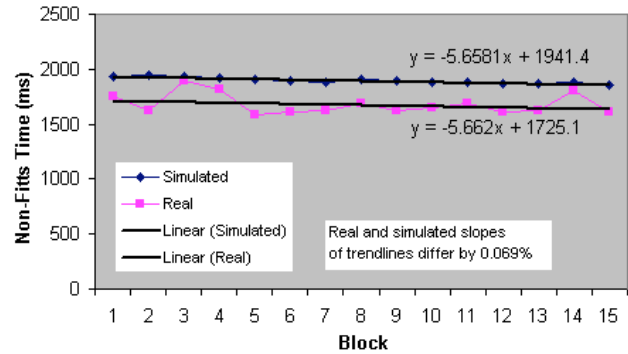
Figure 2. Novice non-Fitts time (simulated vs real) over 15 blocks, 5 trials per block. The slopes of the trendlines for the real and simulated data differ by 0.069%.
