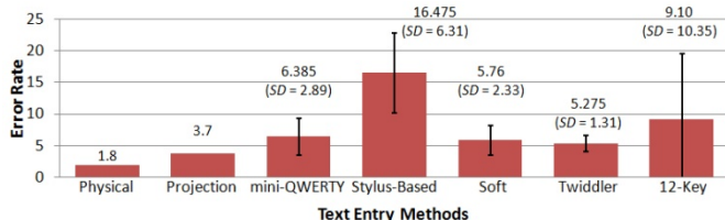
Figure 2. Average error rate for text entry methods.
