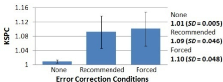
Figure 3. Average KSPC for error correction conditions.
