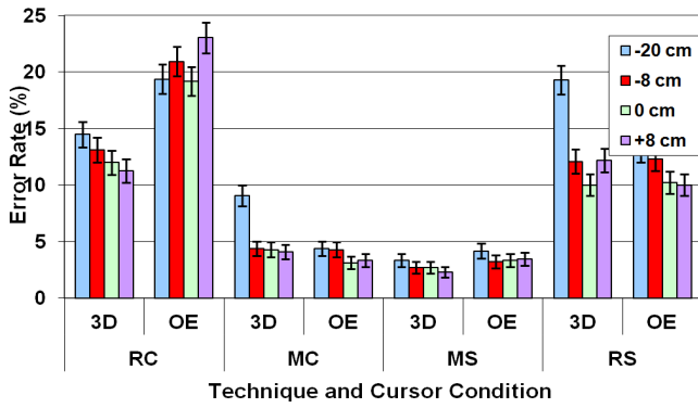
Figure 5. Error rates for each condition. Error bars show \pm 1 standard error
