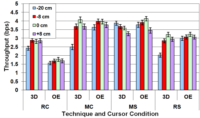
Figure 6. Throughput for each condition. Error bars show \pm 1 standard error. Higher throughput is better.
