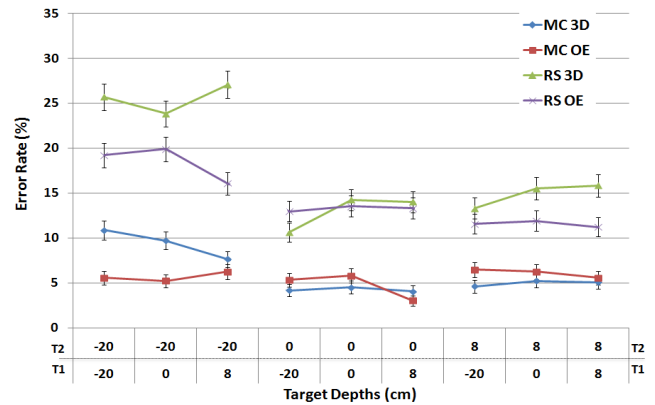
Figure 10. Error rates by technique, cursor style, and depth combination. Error bars show \pm 1 standard error. T1 and T2 are the start and end depths of each trial.
