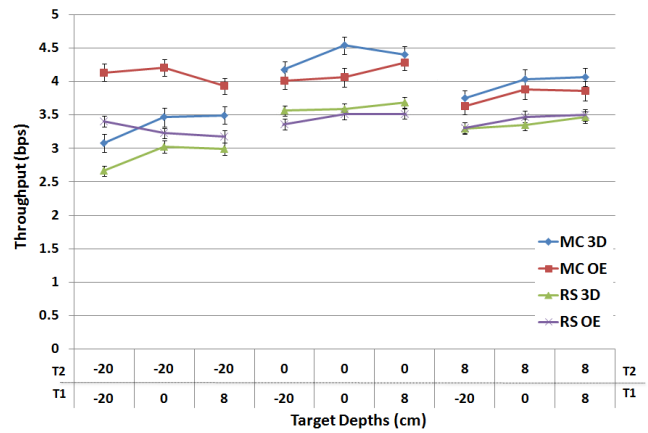
Figure 12. Screen-projected throughput by technique, cursor style, and depth combination. Error bars show \pm 1 standard error. T1 and T2 are the start and end depths of each trial.
