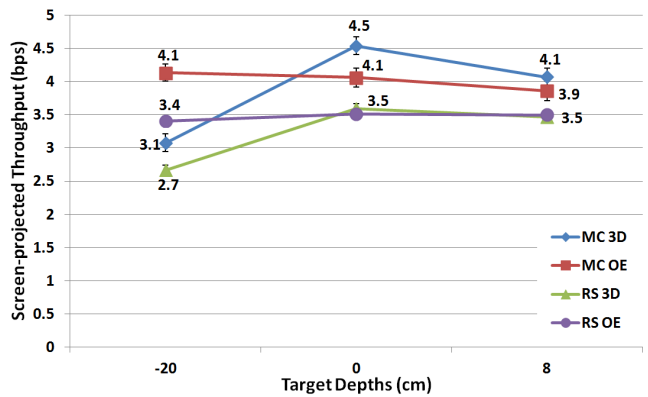
Figure 13. Screen-projected throughput by pointing technique and cursor style for each combination of same-depth targets. Error bars show \pm 1 standard error.
