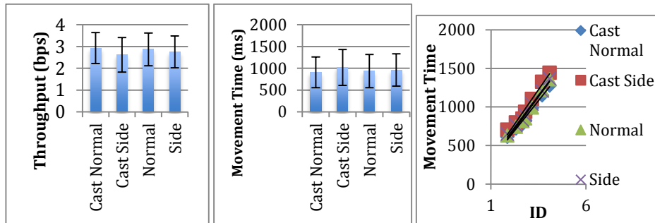
Fig. 4. Graph of average throughput values (left) and movement time (middle) and Fitts’ law model (right) for each condition. Error bars show standard deviation.
